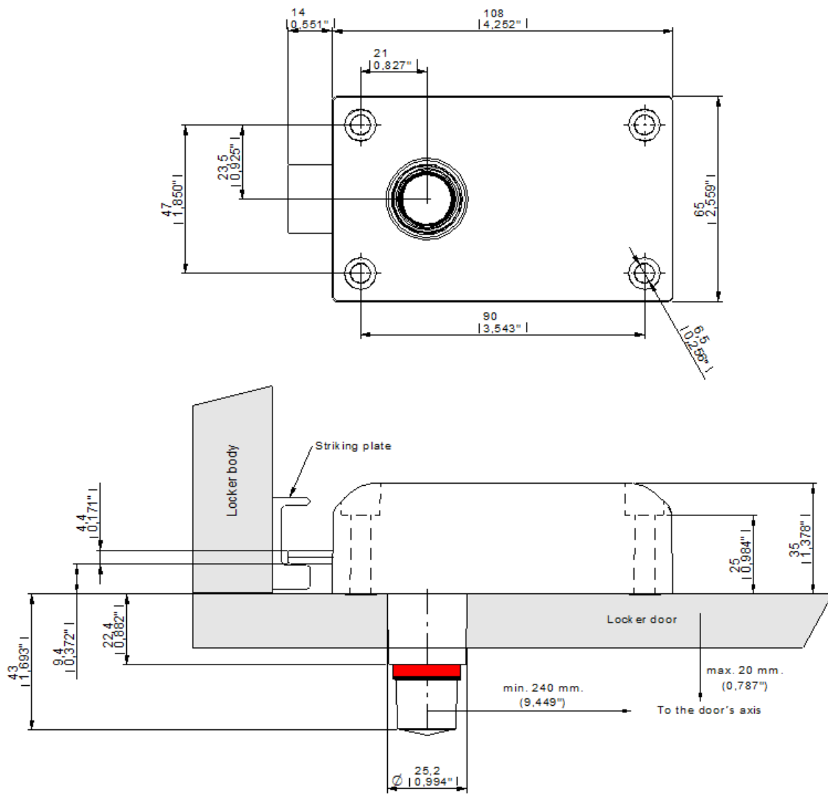
Measurements in mm. (Inches)
